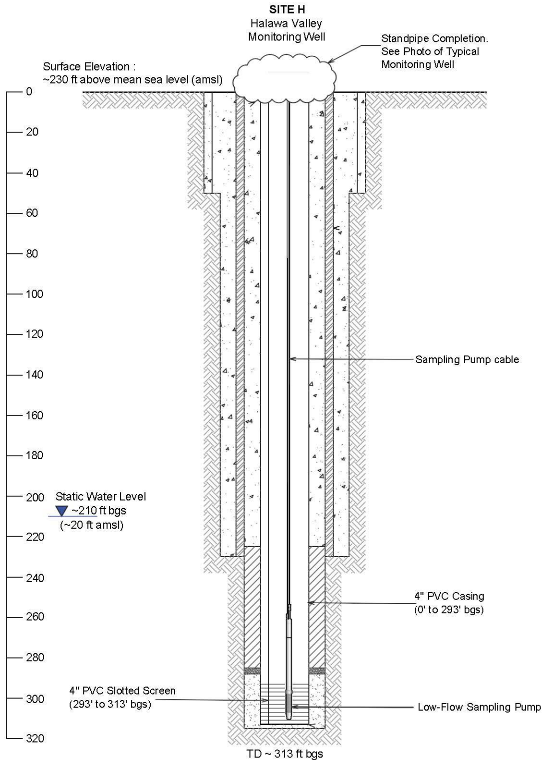
SIMPLIFIED WELL SCHEMATIC NOT TO SCALE
